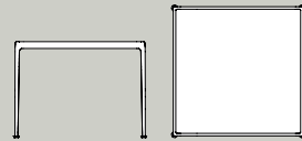
Square Table L 96.5 x D 96.5 x H 72 cm
